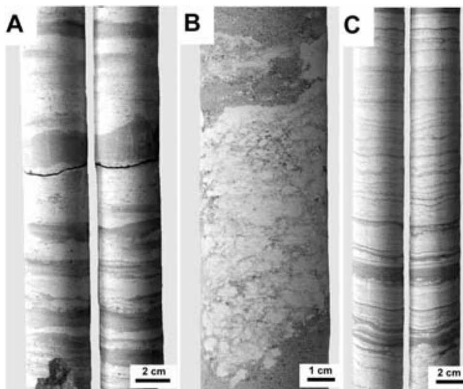
FIGURE 5 | Lithofacies of carbonate and anhydrite. A) Alternation of anhydrite (light) and carbonate (dark) bands; sample at 619.60 m depth. B) Detail of a clastic intercalation (currently anhydritic pseudomorphs or clasts) within the alternation of carbonate and anhydrite bands. Dark material at the top and the base of the intercalation is carbonate; sample at 579.6 m depth. C) Laminated to banded anhydrite (light). Dark material is carbonate laminae; sample at 724.75 m depth.
