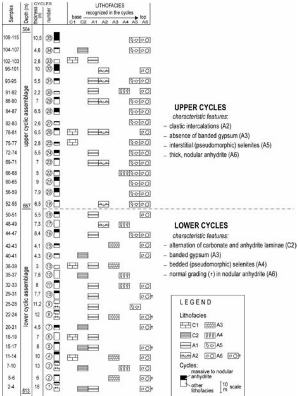
FIGURE 11 Individual cycles found in the evaporitic succession of the Alacón borehole, grouped into two cyclic assemblages.
