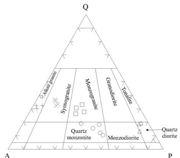
FIGURE 3 | QAP plot of the modal compositions of the plutonic rocks (Streckeisen, 1976). Symbols of the plutonic rocks used in all the given figures are: \Delta = quartz-diorite; \circ = quartz-monzonite; \square = monzogranite; \times = syenogranite; + = alkali feldspar granite.
