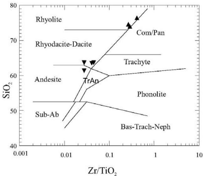
FIGURE 6 | SiO_2 vs. Zr/TiO_2 diagram showing the classification of volcanic rocks (Winchester and Floyd, 1977). Symbols of the volcanic rocks used in all the given figures are: \nabla = Rutig Volcanics; \blacktriangle = Katherina Volcanics.
