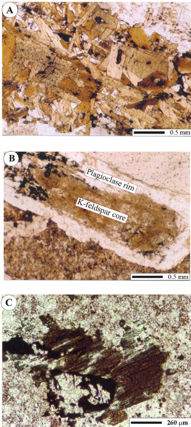
FIGURE 4 | A ) Decussate texture in quartz-diorite (plane light). Note that hornblende recrystallized to an aggregate of actinolite, biotite and chlorite disposed in a criss-cross fashion. B ) Rapakivi texture in monzogranite (plane light). C ) Alkali amphibole phenocrysts in the rhyolite (crossed nichol).
