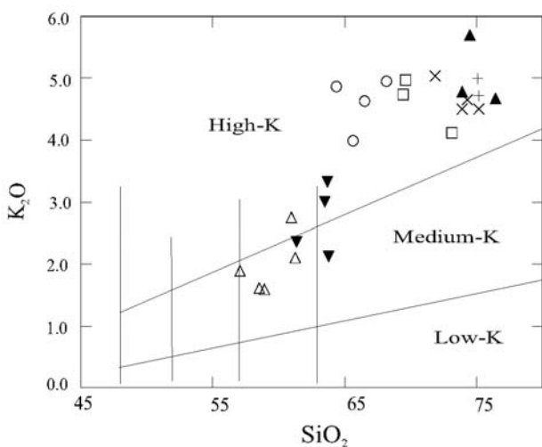
FIGURE 7 | K_2O vs. SiO_2 diagram for the calc-alkaline and alkaline suites (Le Maitre et al., 1989). See legend in Figures 3 and 6.
