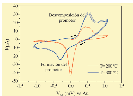
Figura 9. Voltamperogramas c clicos (10 mV/s) en condiciones de reacci n. [\text{NO}] = [\text{C}_3\text{H}_6] = 2000 ppm, [\text{O}_2] = 5\% , caudal total = 12 \text{ l}\cdot\text{h}^{-1} , balance He.
