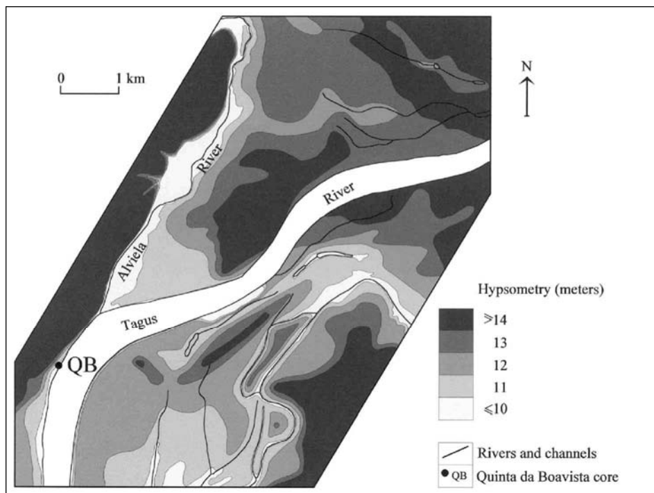
Figure 3 - Morphological frame of Quinta da Boavista site.
