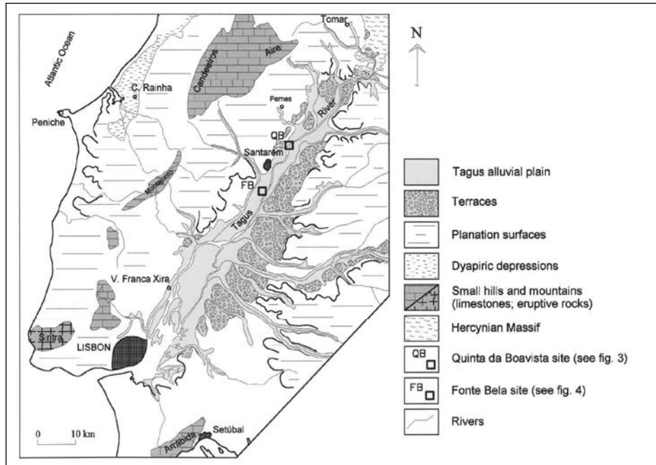
Figure 2 - Geomorphological framework of the Lower Tagus Basin. (D.B. Ferreira, 1980, simplified)
