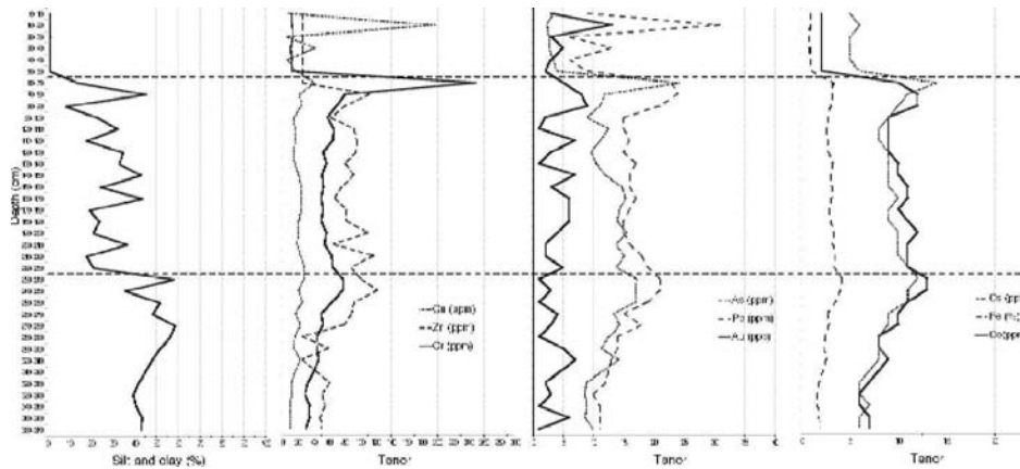
Figure 10 - Heavy metals contents of Quinta da Boavista core.
