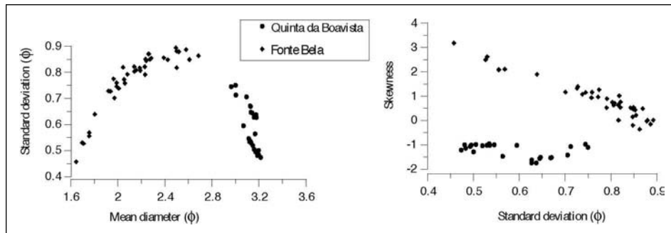
Figure 11 - plot of grain size distribution statistics (sand fraction) of sediments from Quinta da Boavista and Fonte Bela.
