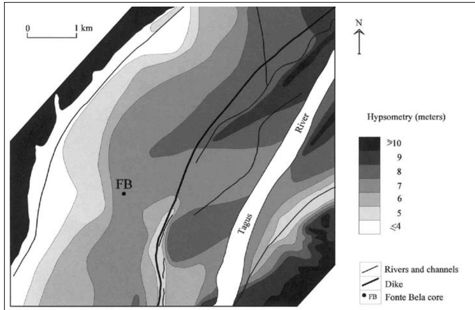
Figure 4 - morphological frame of Fonte Bela site.
