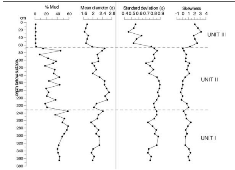
Figure 9 - Vertical profile of Quinta da Boavista core: mud content and extual parameters of sand fraction.
