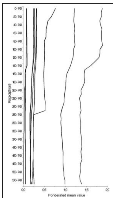
Figure 5 - Geochemical background value definition of the nine heavy metals at Fonte Bela.
