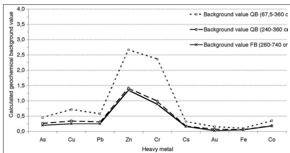
Figure 6 - Comparison of geochemical background values from Fonte Bela (FB) core and those founded in Quinta da Boavista (QB9 core using average values for two different range depths).
