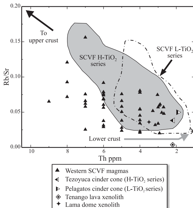
Figure 17. The increase of Rb/Sr and Th with magmatic evolution of the western SCVF magmas suggests magma contamination with upper crustal rather than with lower crustal material. Values of the upper and lower crust from Taylor and McLennan (1985).
