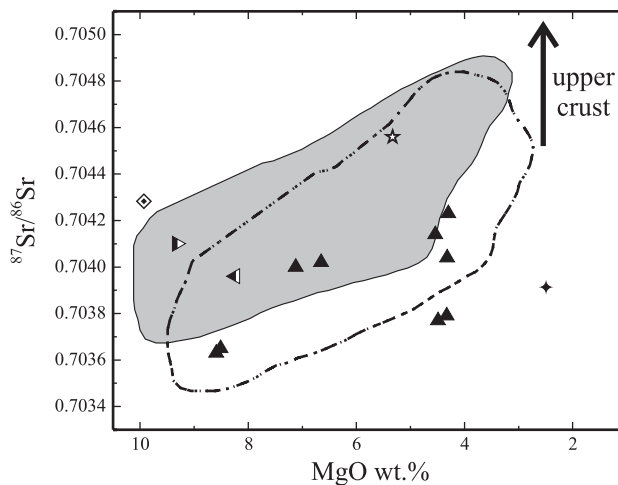
Figure 16. MgO (wt.%) vs. 87 Sr/ 86 Sr diagram for SCVF magmas. The increase of 87 Sr/ 86 Sr ratio with magmatic evolution suggests the occurrence of crustal contamination along with crystal fractionation. Symbols as in Figure 15.
