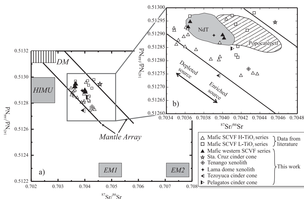
Figure 10. ^{143}\text{Nd}/^{144}\text{Nd} vs. ^{87}\text{Sr}/^{86}\text{Sr} for mafic volcanic rocks ( \text{MgO} \geq 6.0 wt.%), Sta Cruz cinder cone and crustal xenoliths of the Tenango area. a) DM: Depleted mantle; EMI: enriched mantle 1; EM2: enriched mantle 2; HIMU: high ^{238}\text{U}/^{204}\text{Pb} mantle; data from Zindler and Hart (1986). b) The gray-filled area represents the isotopic ratios of nearby Nevado de Toluca volcano (NdT), whereas the area filled with the line pattern represents data from Popocatepetl volcano. Data provenance: Verma (2000); Velasco-Tapia (2002); Martínez-Serrano et al. , 2004, Siebe et al. (2004b) and Schaaf et al. (2005).
