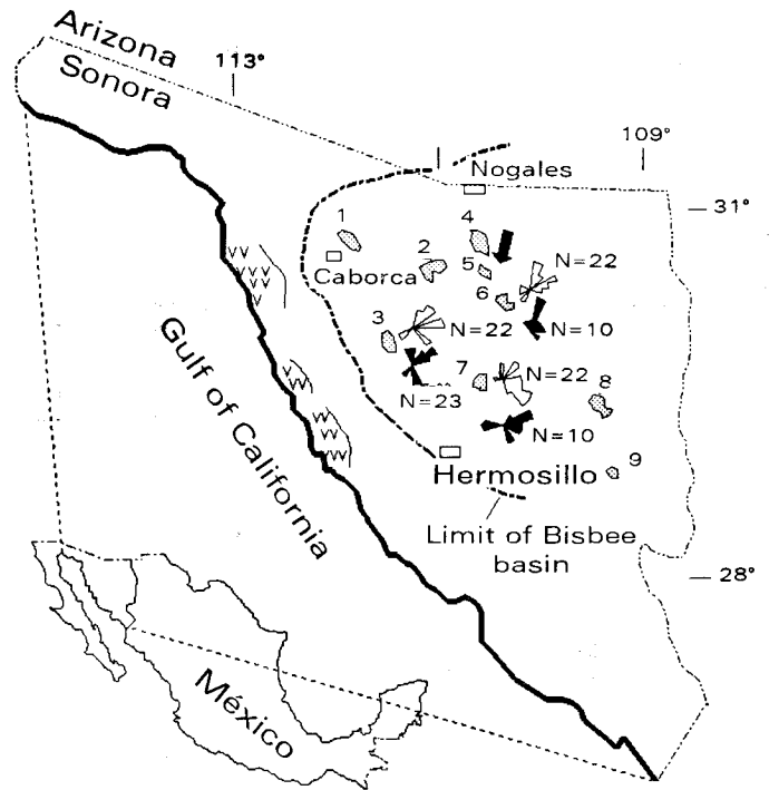
Figure 1.- Locations of Lower Cretaceous outcrops mentioned in the text: 1, sierra El Chanate; 2, Santa Ana area; 3, Cerro Mayo; 4, sierra El Pinito; 5, Cerro Azul; 6, Arizpe; 7, Cerro de Oro; 8, Lampazos; 9, Arivechi. Also shown are paleocurrent directions of the Gance Conglomerate, Morita (filled in black) and Cintura (filled in white) Formations; outcrops of Lower Cretaceous volcanics along the coast of Sonora, and inferred limits of the Bisbee basin. Paleocurrent directions from the Gance Conglomerate in sierra El Pinito taken from Gilmont (1979).
