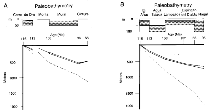
Figure 4.- Curves indicating total subsidence (dashed curve), and minimum and maximum tectonic subsidence curves (solid curves) from the (A) Cerro de Oro and (B) Lampazos areas. Also shown is estimated paleobathymetry for each formation. Geologic time scale from Haq et al. , 1988.
