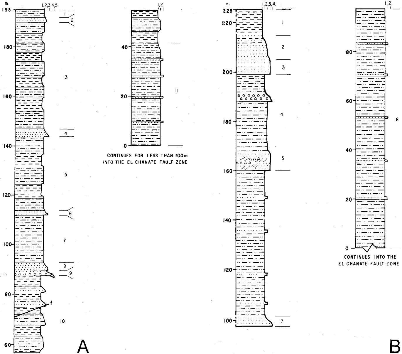
Figure 8.- (A) Measured stratigraphic column of section II; and (B) measured stratigraphic column of section III. For their location see Figure 5. Notes same as in Figure 6.
