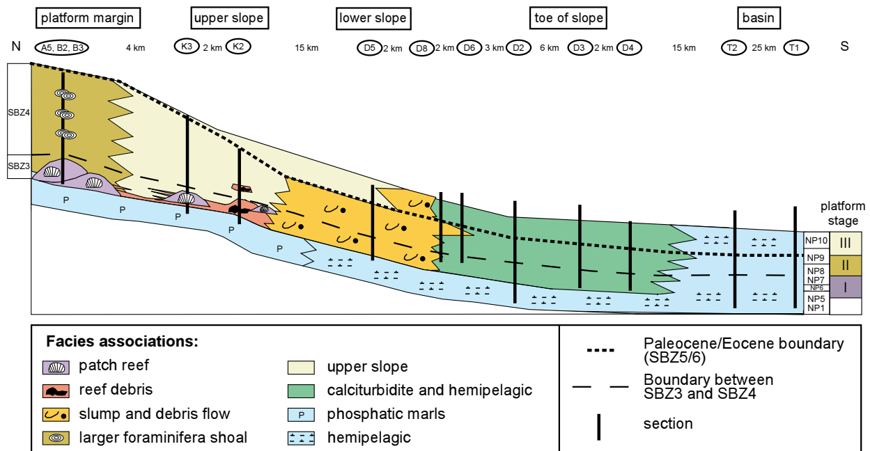
FIGURE 4 | Platform-basin transect of the Paleocene to Lower Eocene in the Galala Mountains (Egypt) with biostratigraphic zonation and platform stages.
