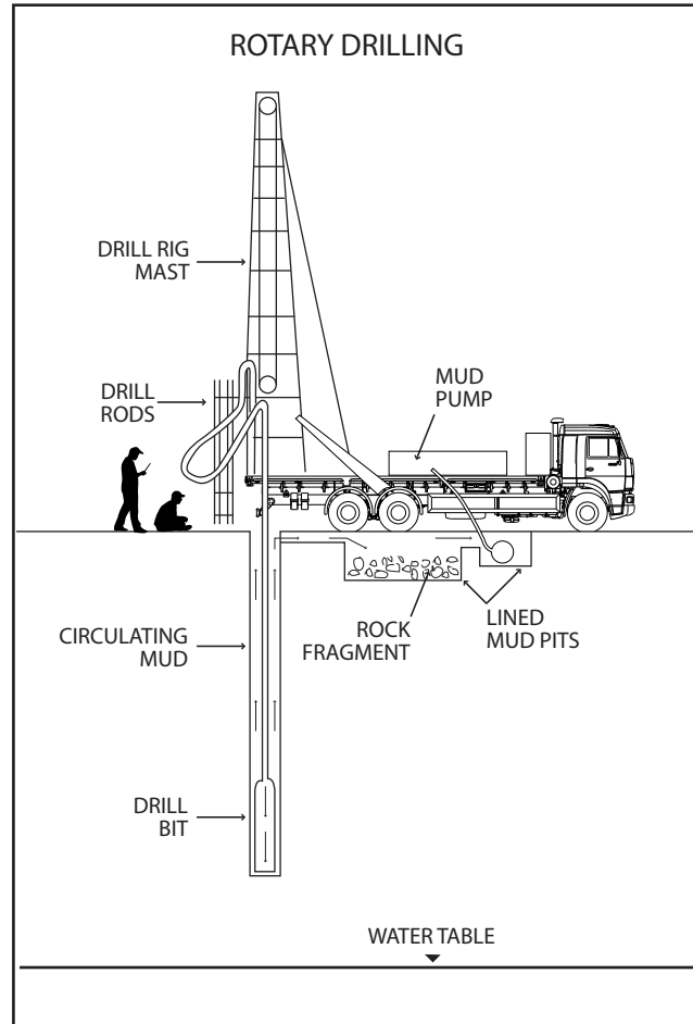
Figure 4. Typical layout for a rotary drilling
