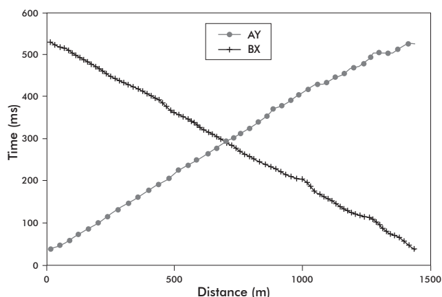
Figure 10. First arrivals obtained from the line 1040
