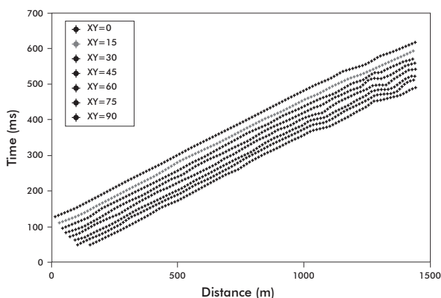
Figure 11. Velocity analysis for XY values from 0 to 90 m. These data come from the first arrival times in Figure 8
