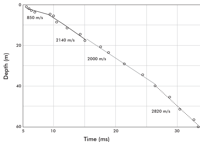
Figure 7. Downhole B First arrivals and Velocity model
