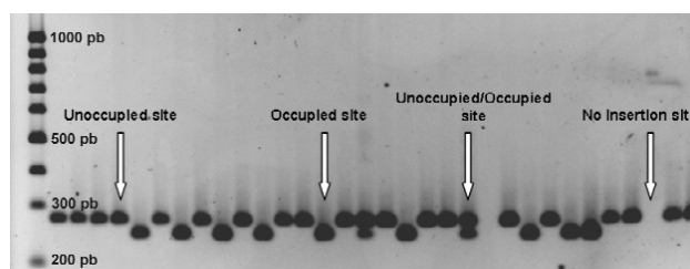
Figure 1. Agarose gel (1.5%) showing three different alleles of the RBIP locus 28Lx1. Numbers indicate the reference size markers in base pairs.
