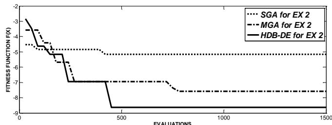
Fig.8. Convergence curve for EX 2 consists of 5 hexagonal cells with 17 channels.
