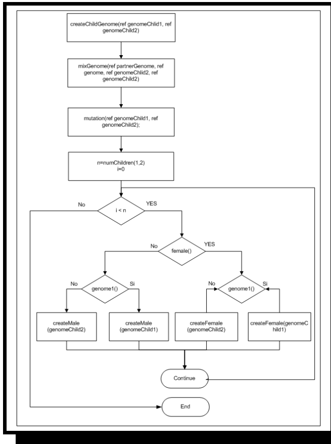
Figure 6 giveBirth() function
