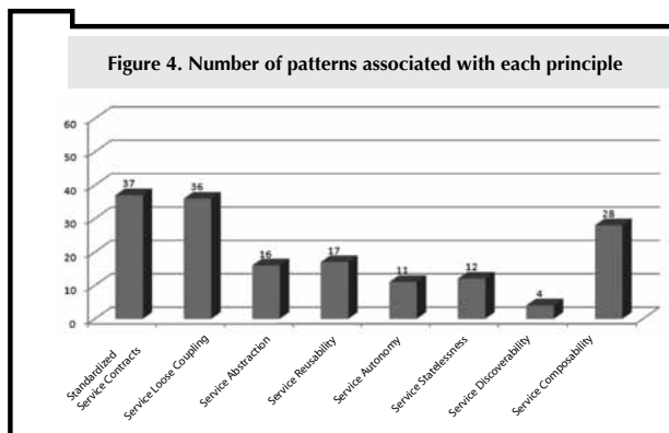
Figure 4. Number of patterns associated with each principle
