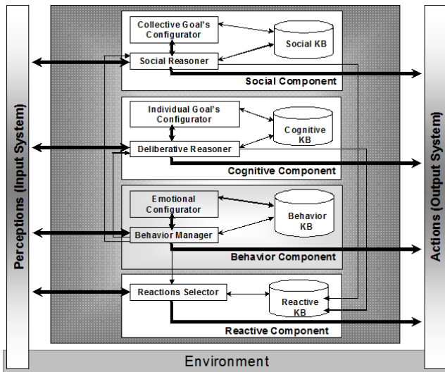
Figure 3: Components of MASOES at Individual Level.
