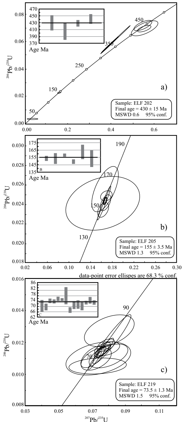
Figure 5. Concordia diagram and weighted-average ages of (a) Realito Gabbro; (b) Topaco Formation; (c) Guamuichil Formation.
