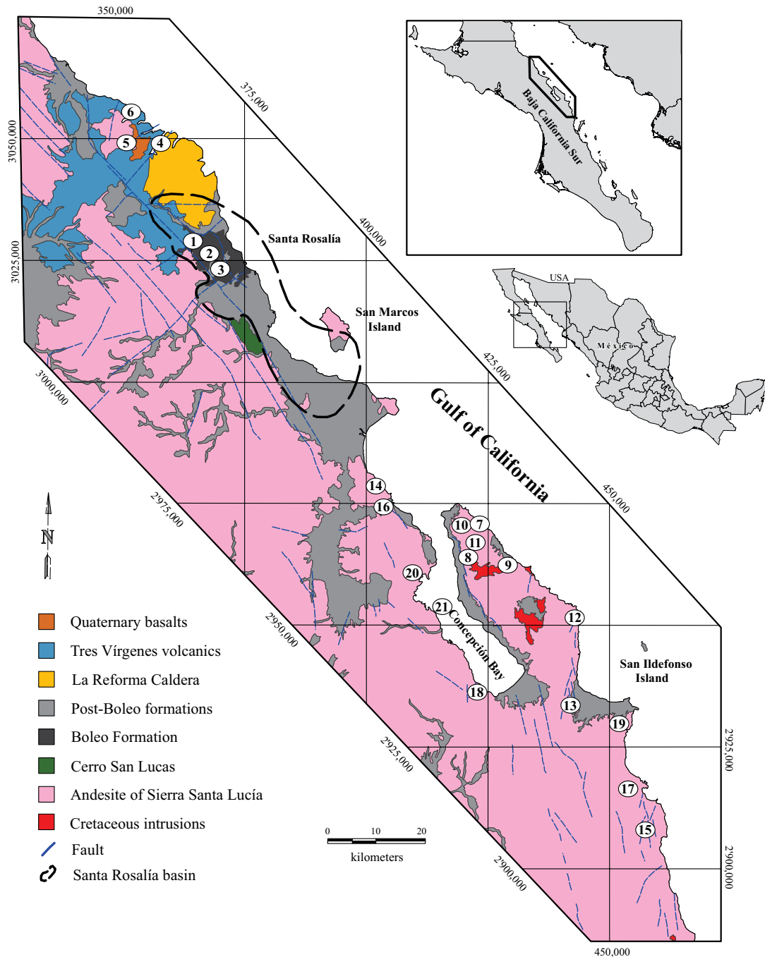
Figure 1. Simplified geological map showing the location of Cu-Co-Zn Boleo district, and other copper and manganese deposits in Baja California Sur, Mexico (modified after Conly et al. 2006; Del Rio Salas, 2011). Localities: (1) Lucifer, (2) Neptuno area, (3) Boleo, (4) San Alberto, (5) Rosario, (6) Caracol, (7) Gavilán, (8) Mantitas, (9) La Trinidad, (10) Pilares, (11) Las Minitas, (12) Santa Teresa, (13) Santa Rosa, (14) Las Delicias, (15) Mencenares volcanic field, (16) Mulegé, (17) San Juanico, (18) Azteca, (19) Saquicisumde and Los Volcanes, (20) Santispac, (21) Mapachitos.
