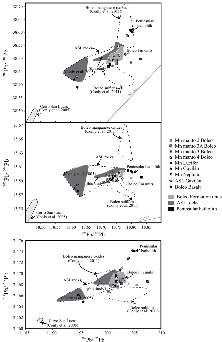
Figure 5. Diagrams showing the lead isotope ratios for the manganese mineralization from the different mineralized mantos and the manganese deposits around Santa Rosalía. ASL: Andesite of Sierra Santa Lucía; NHRL: Northern Hemisphere Reference Line.
