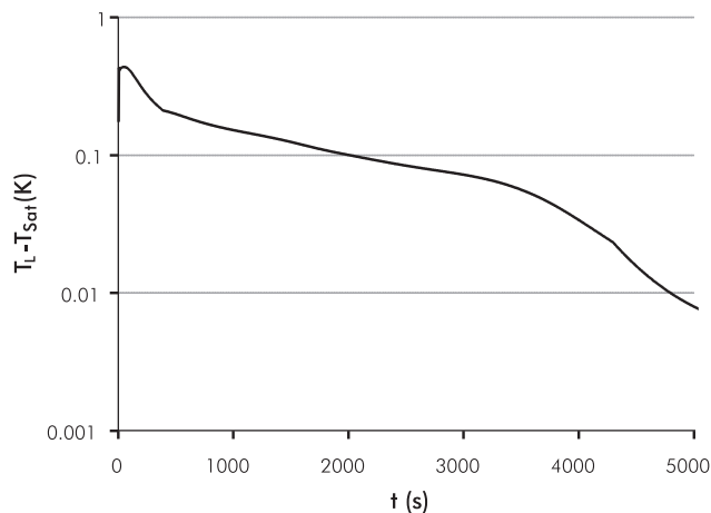
Figure 11. Difference between liquid phase temperature and saturation temperature (evaluated at saturation pressure).
