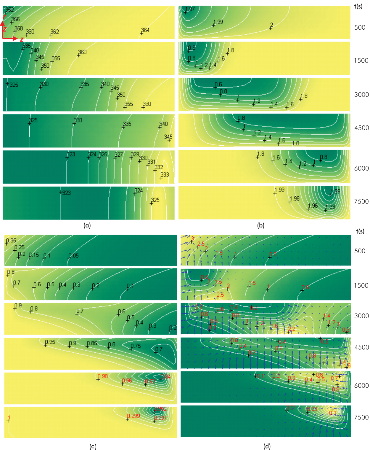
Figure 9. Instantaneous contour plots for (a) RM temperature (units in K); (b) gas pressure (units in bar); (c) reaction conversion; (d) reaction rate (units in \text{mol}\cdot\text{m}^{-3}\cdot\text{s}^{-1} ) and velocity field.
