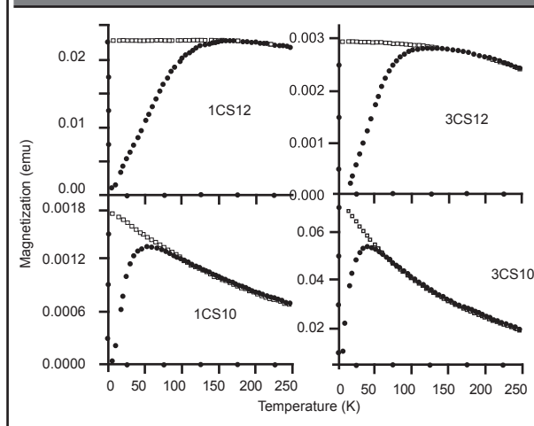
Figure 9. FC (squares) and ZFC (solid dots) magnetization curves versus temperature for the samples
