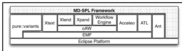
Figure 1. High-level MD-SPL framework architecture.
