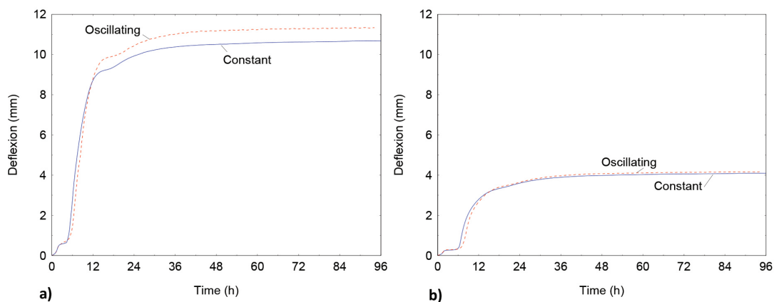
Figure 6. Evolution of the deflexion of flatsawn (a) and quartersawn boards (b) dried with constant or oscillating conditions (10 mm thick) ( Experimental results ).
