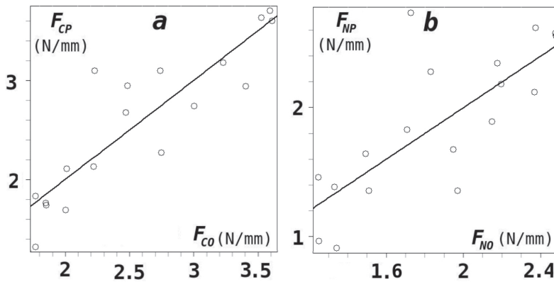
Figure 7. For up- routing of Oak ( Quercus petraea ): a) plot of the main cutting force observed F_{CO} against the main cutting force predicted F_{CP} according to equation (3), b) plot of the normal force observed F_{NO} against normal force predicted F_{NP} , according to equation (4).
