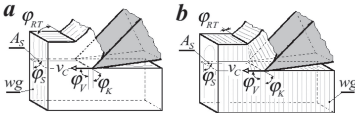
Figure 3. Orientation angles between wood grain (wg) and: v_C - vector of cutting velocity; k - cutting edge; A_S - cutting plane; for perpendicular cutting case ( \varphi_K=90^\circ , \varphi_V=90^\circ , \varphi_S=90^\circ ); by growth rings orientation angle \varphi_{RT} : a - \varphi_{RT}=90^\circ (radial); b - \varphi_{RT}=0^\circ (tangential); A_S - cutting plane.
