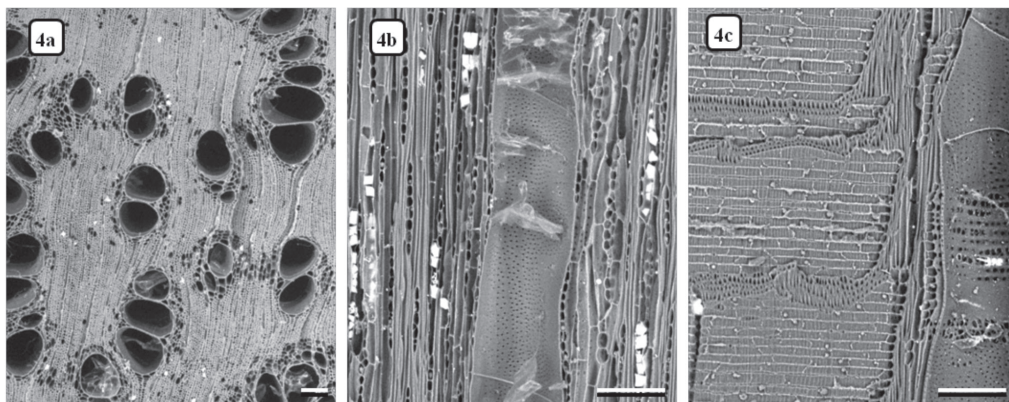
Figure 4. Plate 4. Eucalyptus microcorys . Charcoal micrographs. Sections (a) Transverse, (b) Tangential Longitudinal, (c) Radial Longitudinal. Bars: 100 \mu m.
