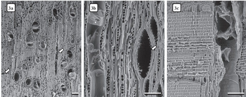
Figures 3. Plate 3. Eucalyptus dunnii . Charcoal micrographs. Arrows show the ruptures. Sections (a) Transverse, (b) Tangential Longitudinal, (c) Radial Longitudinal. Bars: 100 \mu m.
