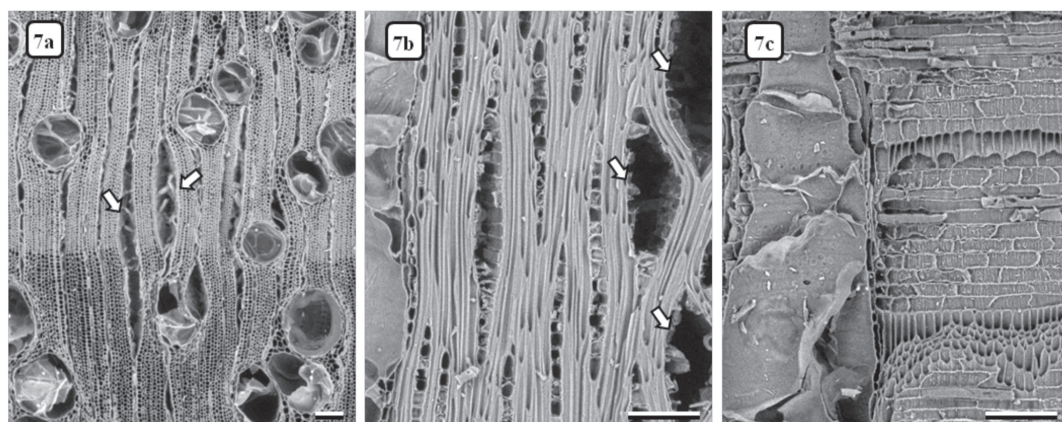
Figure 7. Plate 7. Eucalyptus viminalis . Charcoal micrographs. Arrows show the ruptures. Sections (a) Transverse, (b) Tangential Longitudinal, (c) Radial Longitudinal. Bars: 100 \mu m.
