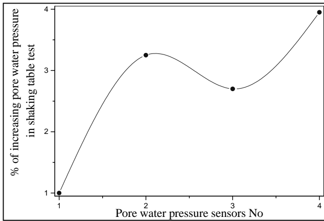
Figure 4. Detail of pore pressure characteristics
