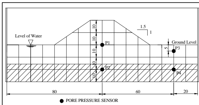
Figure 3. Position of transducer during the shaking table test (Namdar, 2009)
