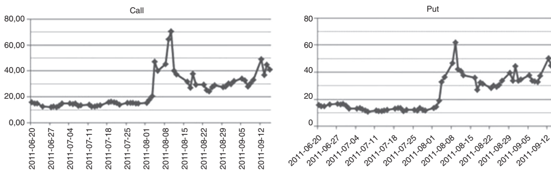
Fig. 3. Implied volatilities (in %) curves for call (left) and put (right) options with expiring day of 16.09.2011 calculated for at-the-money points.
