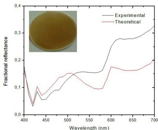
Figure 6 Experimental and theoretical diffuse reflectance of sample 6
