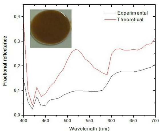
Figure 6 Experimental and theoretical diffuse reflectance of sample 6
