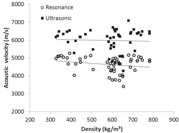
Figure 2. Relationship between acoustic velocity with wood density.
