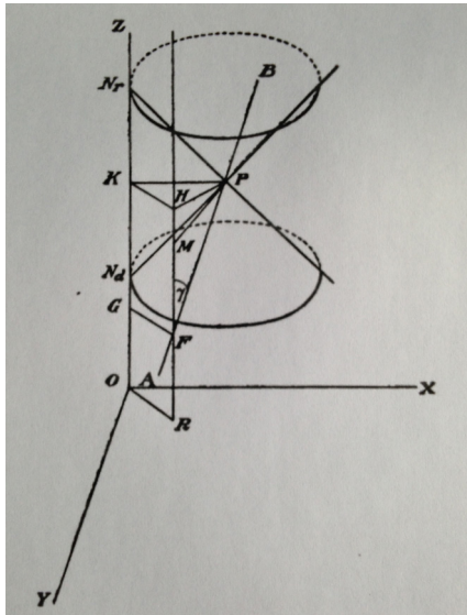
Figure 4. Robb's light cones (1911).
