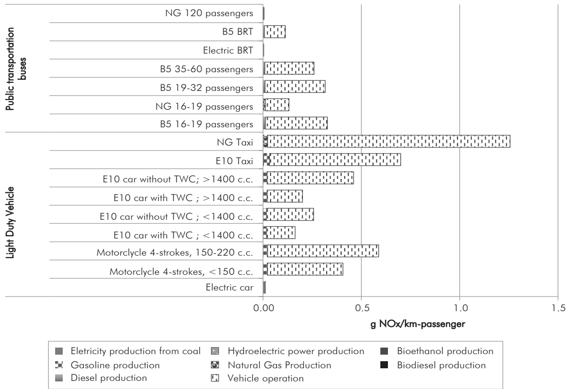
Figure 7. Well-to-wheel NOx emissions from selected energy sources of the vehicle categories. (g/km-passenger). NG: natural gas; BRT: Bus Rapid Transit; B5: blend 5% biodiesel-diesel; E10: blend 10% bioethanol-gasoline; TWC: Three-way catalyst.
