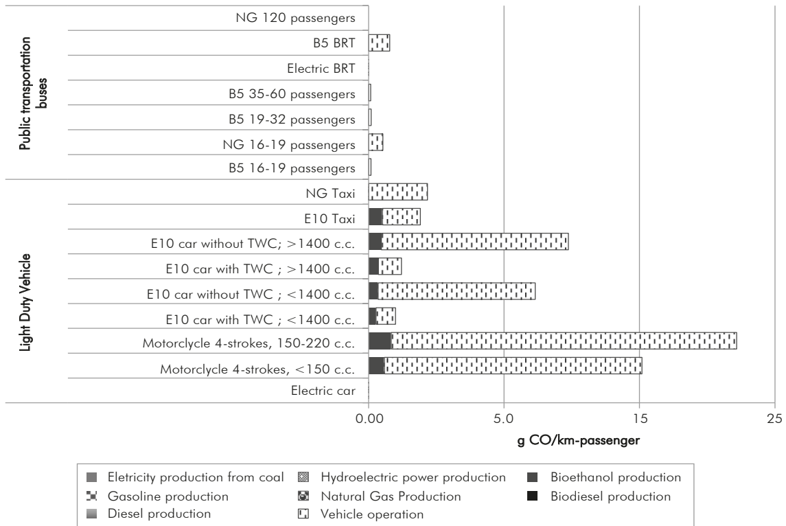
Figure 6. Well-to-wheel CO emissions of selected energy sources of the vehicle categories. (g/km-passenger). NG: natural gas; BRT: Bus Rapid Transit; B5: blend 5% biodiesel-diesel; E10: blend 10% bioethanol-gasoline; TWC: Three-way catalyst.
