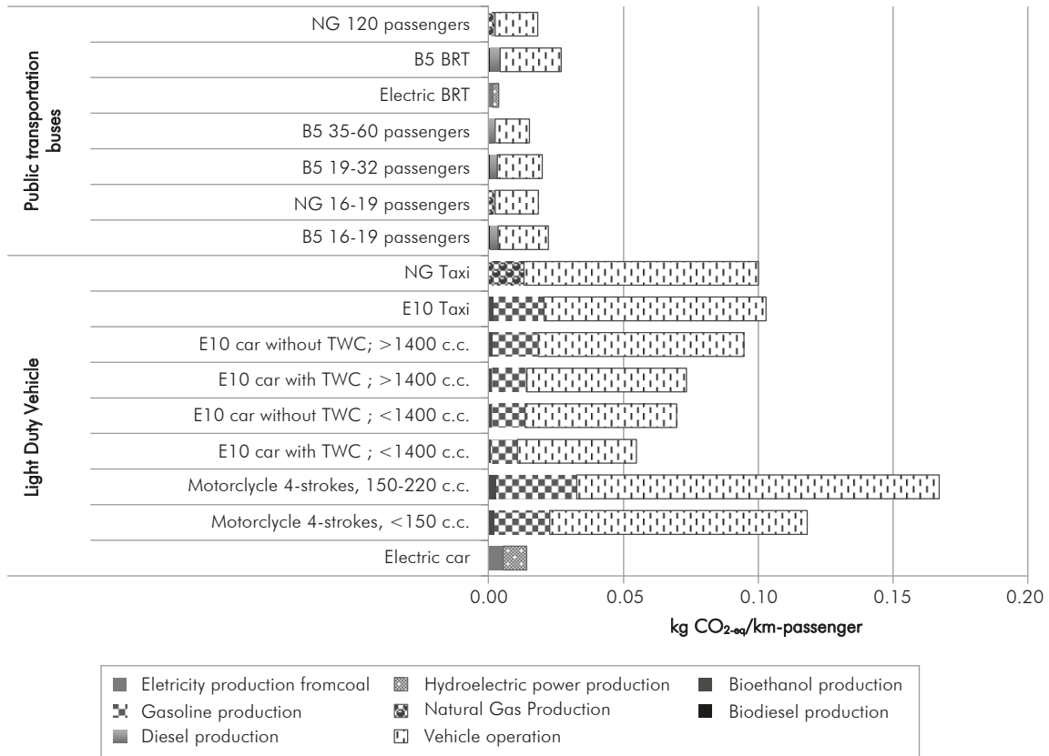
Figure 4. Well-to-wheel CO 2-eq emissions from selected energy sources of the vehicle categories. (kg/km-passenger). NG: natural gas; BRT: Bus Rapid Transit; B5: blend 5% biodiesel-diesel; E10: blend 10% bioethanol-gasoline; TWC: Three-way catalyst.
