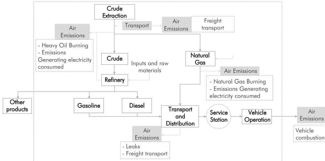
Figure 1. System Boundaries for fossil fuels.
