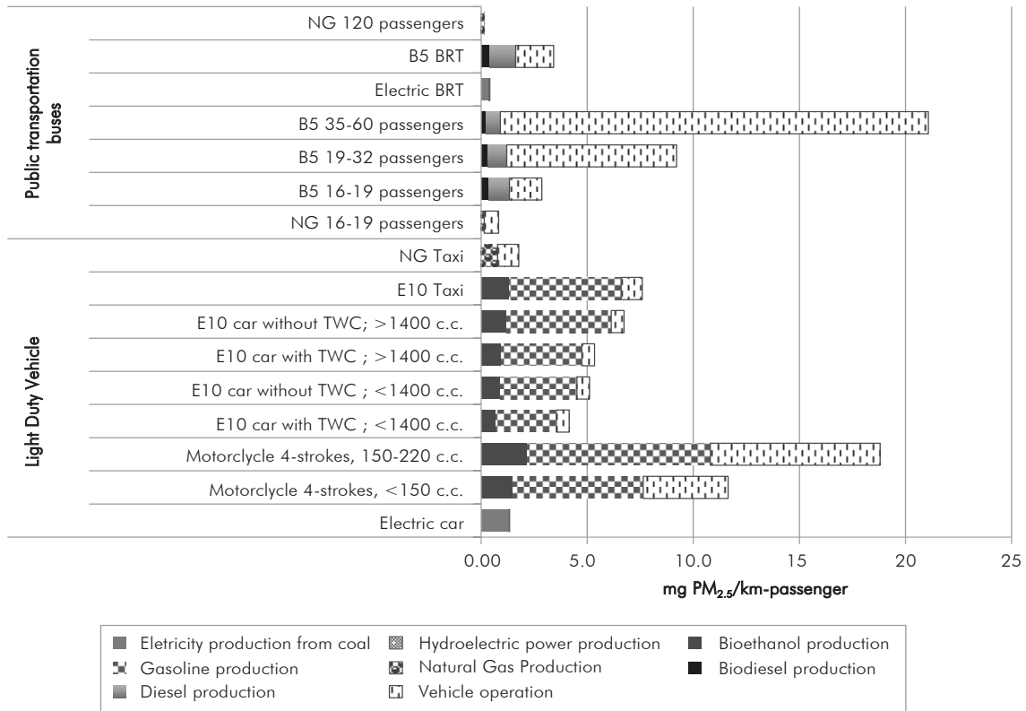
Figure 5. Well-to-wheel PM 2.5 emissions from selected energy sources of the vehicle categories. (mg/km-passenger). NG: natural gas; BRT: Bus Rapid Transit; B5: blend 5% biodiesel-diesel; E10: blend 10% bioethanol-gasoline; TWC: Three-way catalyst.
