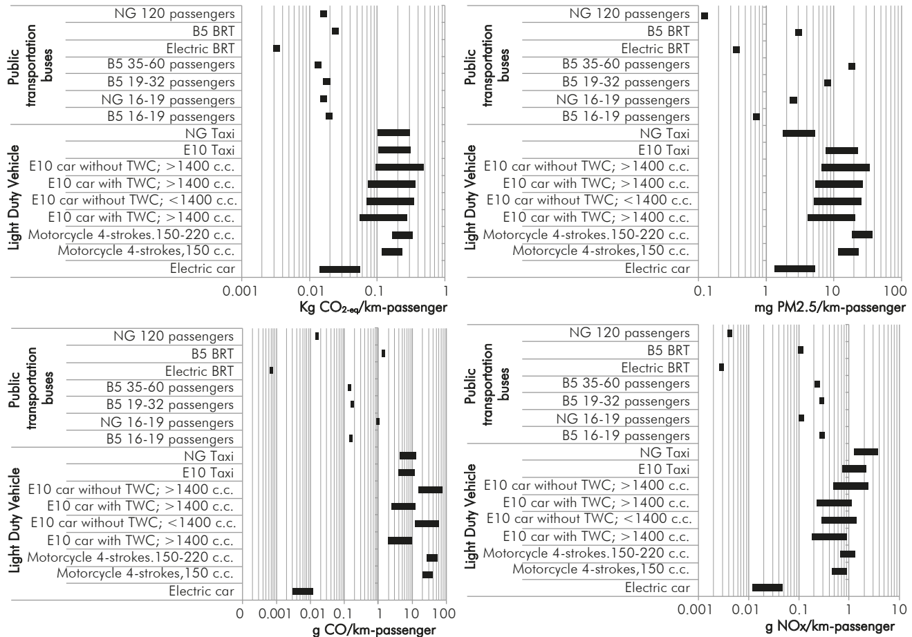
Figure 8. Impact of vehicle occupancy on the estimated WTW emissions. Light duty vehicles: emissions were estimated at design and minimum occupancy (only one passenger). Public transport buses: emissions were estimated at their design occupancy and 25% overcrowding. NG: natural gas; BRT: Bus Rapid Transit; B5: blend 5% biodiesel-diesel; E10: blend 10% bioethanol-gasoline; TWC: Three-way catalyst.
