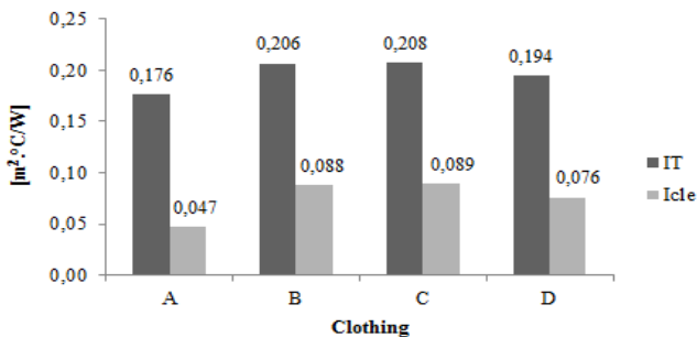
Figure 4. Total thermal insulation and effective clothing insulation of scrub and clean air suits.
