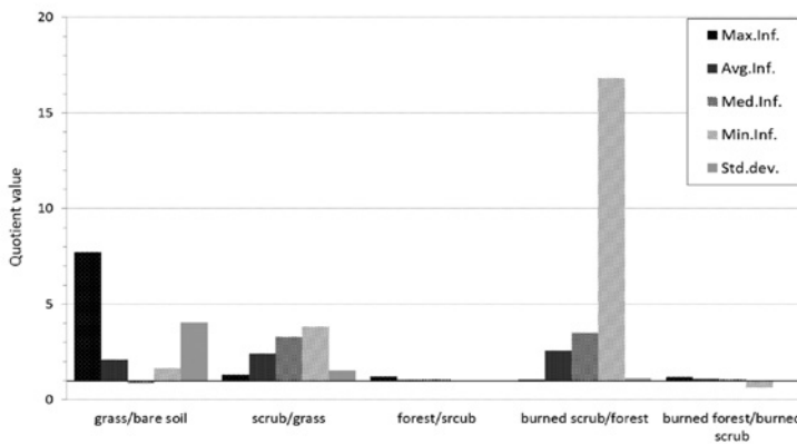
Figure 7. Quotient between the statistic descriptors of infiltration from correlative vegetation groups, following the order shown in Figure 6.
