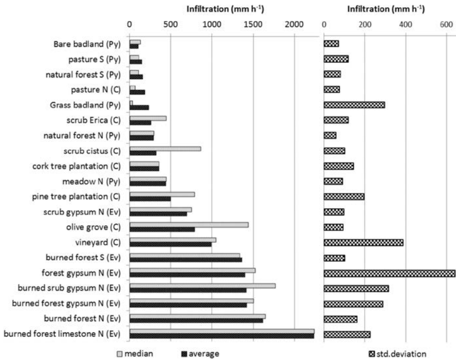
Figure 2. Average, median and standard deviation values of infiltration rates. Land uses are ranked from low to high average infiltration values. Py: Pyrenees/Jaca; C: north-eastern coast/Cap de Creus; Ev: Ebro valley/Zuera.
