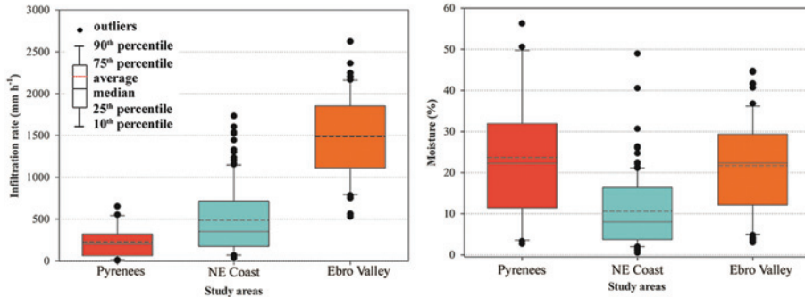
Figure 3. Results of 195 infiltration test for the respective study sites. (A) Infiltration rates ( \text{mm h}^{-1} ). (B) Moisture (%).
