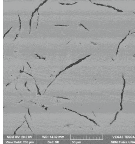
Figure 1. Micrograph of gray cast iron without biodiesel exposure. 2000X. Polished with alumina 10 \mu\text{m} . Lamellar graphite with pearlitic phase in the matrix.
