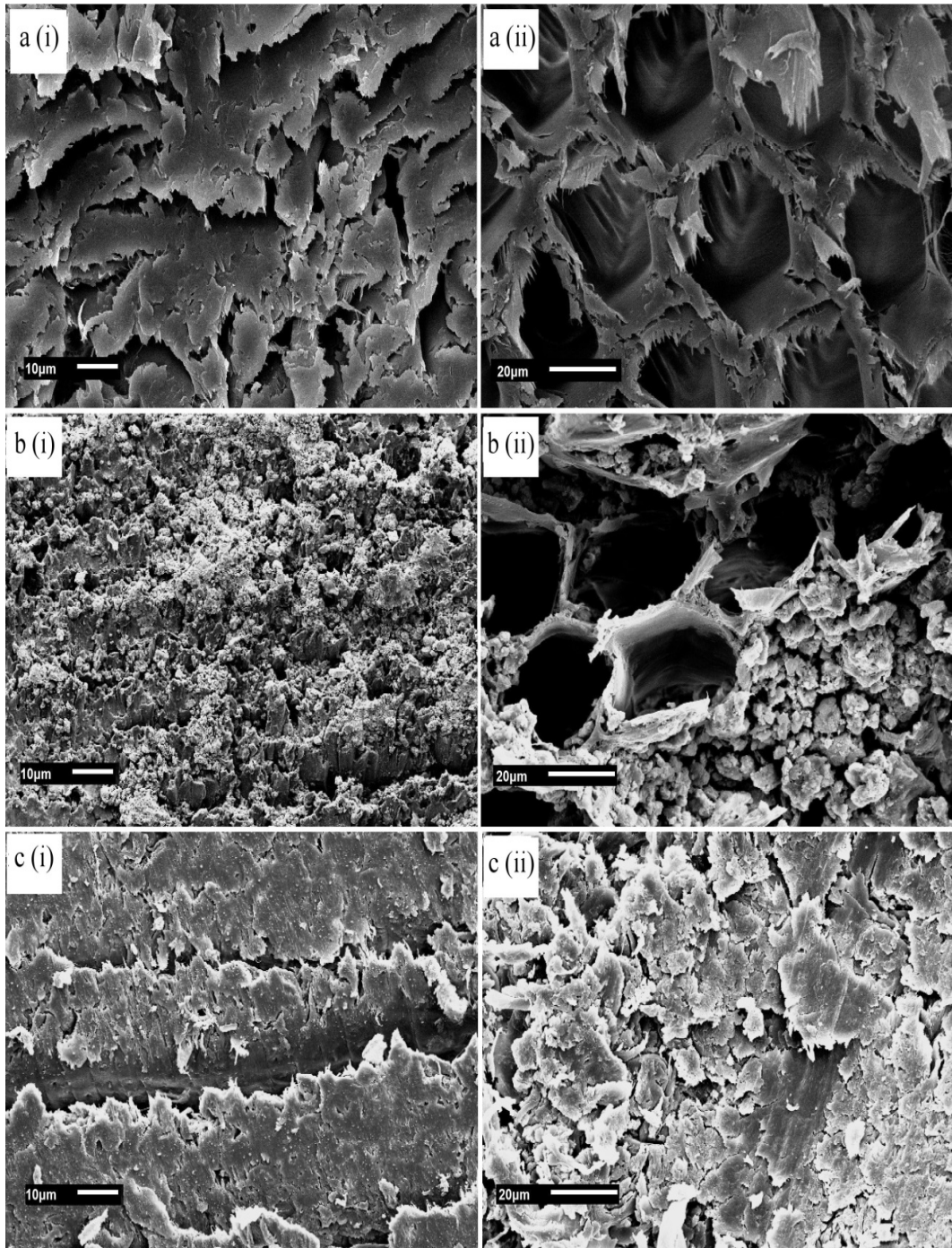
Figure 3. SEM images of untreated Pinus elliotii wood (a), wood impregnated with TiO 2 by vacuum-pressure (b) and wood impregnated with TiO 2 by simple immersion (c). Where: (i) wood surface; (ii) wood tracheids.
