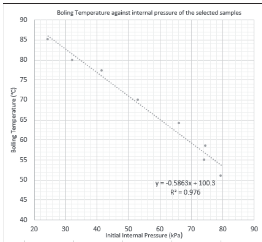
Figure 6: Boiling Temperature against internal pressure of the selected samples Source: Authors, Microsoft Excel graph.
