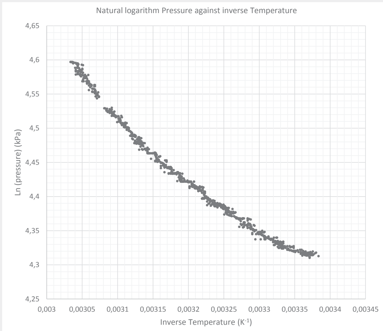
Figure 3: Natural logarithm pressure against inverse Temperature Source: Authors, Microsoft Excel graph.
