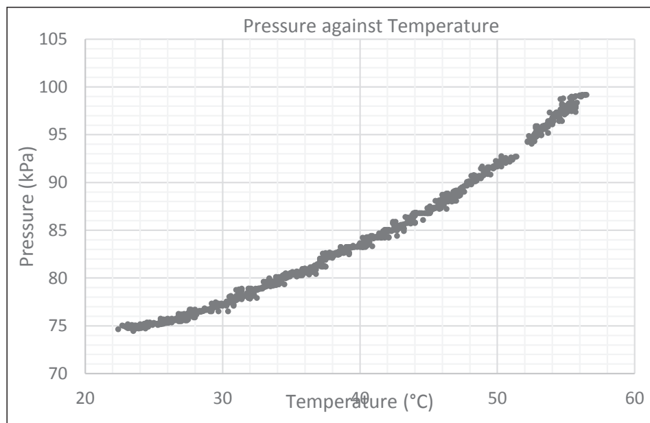
Figure 2: Pressure against Temperature Source: Authors, Microsoft Excel graph.
