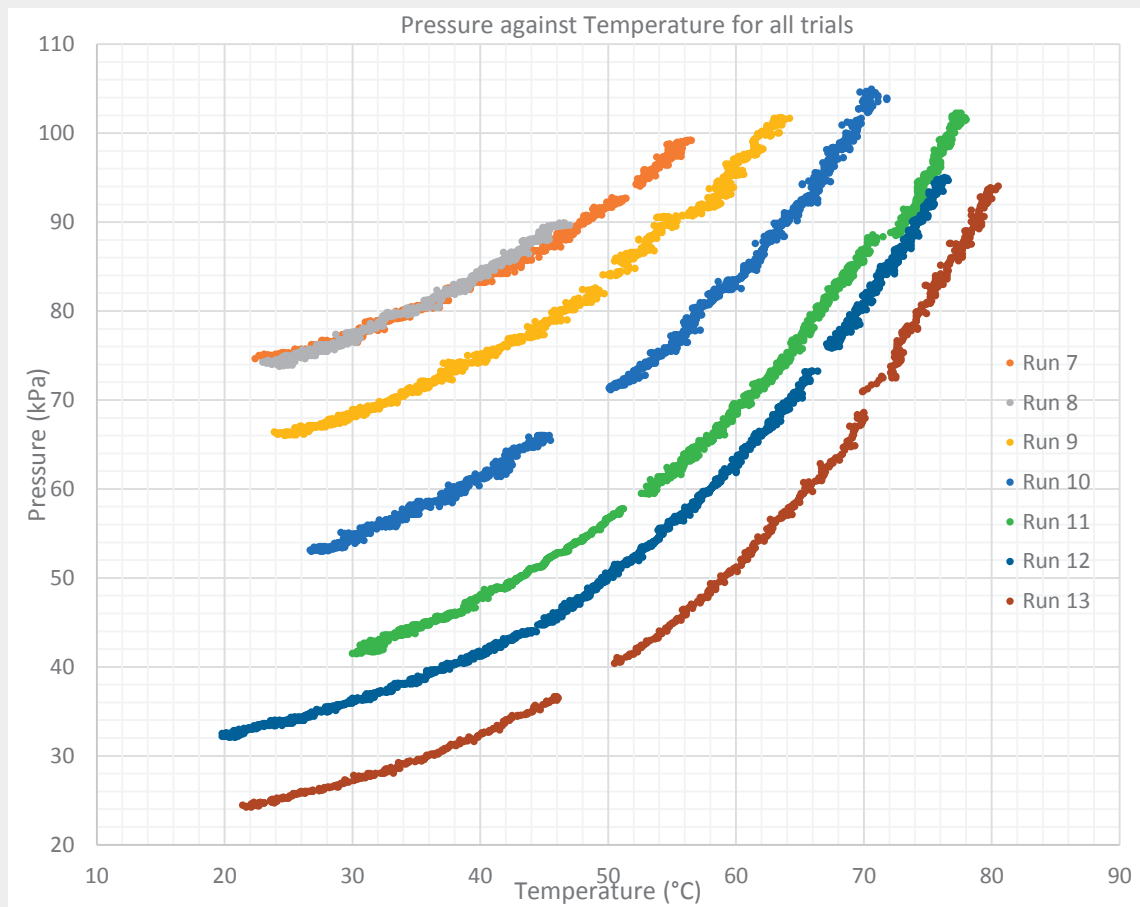
Figure 5: Pressure against Temperature for all selected trials Source: Authors, Microsoft Excel graph.
