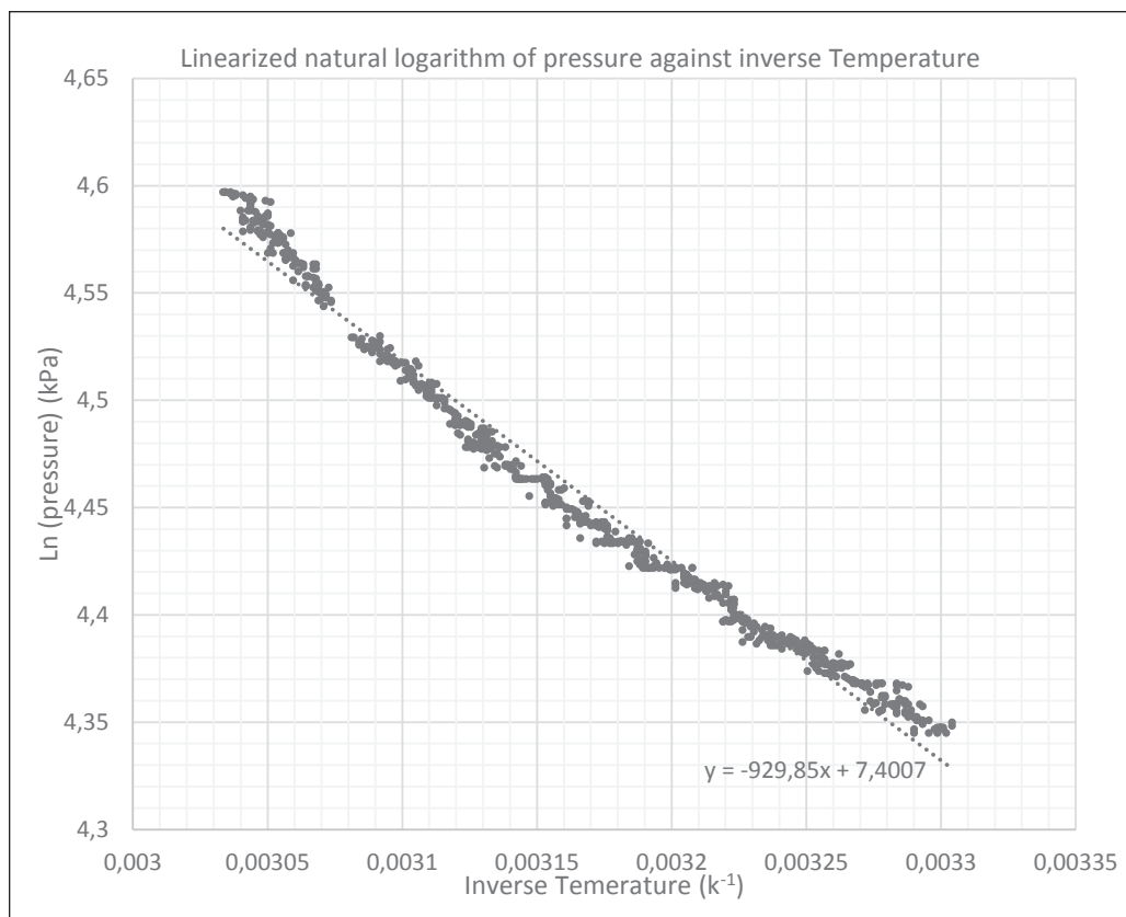
Figure 4: Linearized natural logarithm pressure against inverse Temperature Source: Authors, Microsoft Excel graph.
