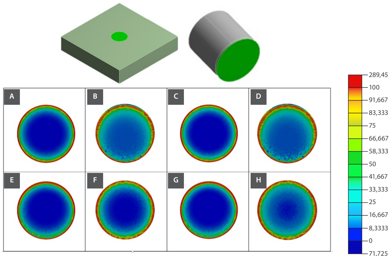
Figure 3. Results of shear and tensile stress at the surface of the resin cylinder and the ceramic for both groups. (a) shear stress at the surface of the ZLS, (b) tensile stress at the surface of the ZLS, (c) shear stress at the surface of the YZHT, (d) tensile stress at the zirconia surface, (e) shear stress in the cement on the ZLS, (f) tensile stress in the cement on the ZLS, (g) shear stress in the cement on the YZHT and (h) the tensile stress in the cement on the YZHT.
