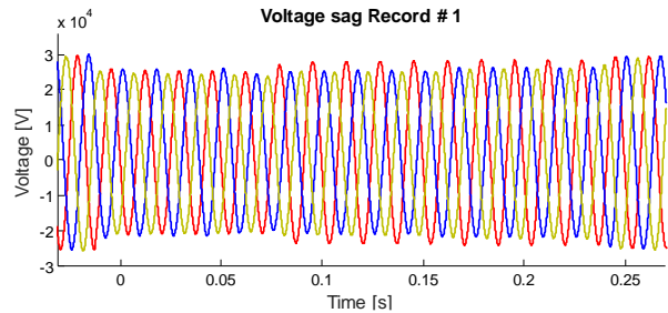
Figure 8. Multistate sag - record 1. Source. Own elaboration.
