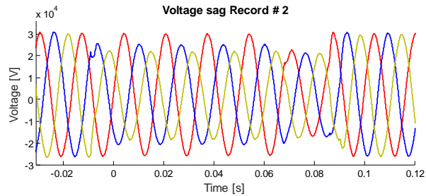
Figure 9. Multistate sag - record 2. Source. Own elaboration.
