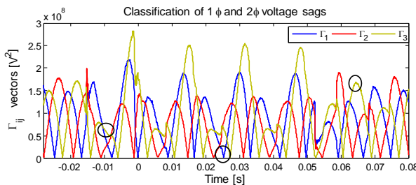
Figure 6. \Gamma_{ij} vectors multistate sag. Source. Own elaboration.
