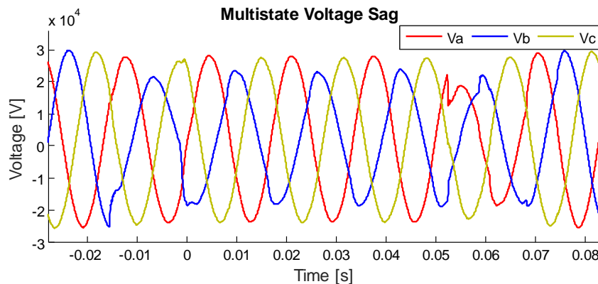
Figure 1. Multistate voltage sag. Source. Own elaboration.
