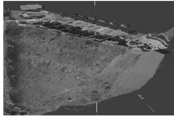
Figure 8. Three-dimensional model of the slope. Failure mechanism. Source: The authors.
