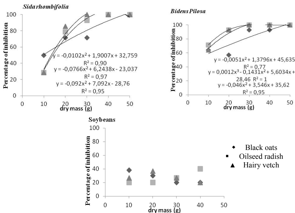
Figure 1. Inhibition percentage of Bidens pilosa , Sida rhombifolia and soybean under black oats, oilseed radish and hairy vetch.
