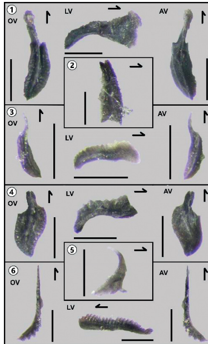
Figure 3. Some of the most representative conodonts found in this study. 1 – Polygnathus costatus , sample CAB-E 1. 2 – Belodella sp. 1, sample CAB-E 5. 3 – Polygnathus sp. 1, sample CAB-E 10. 4 – Polygnathus trigonicus , sample CAB-E 11. 5 – Belodella sp. 2, sample CAB-E 10. 6 – Tortodus australis , sample CAB-E 12. OV = oral view; LV = lateral view; AV = aboral view. Arrows indicate anterior end. Scale = 0.5 mm.
