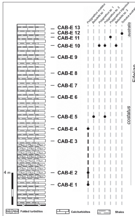
Figure 2. Simplified stratigraphic log with the location of each sample in the sequence and respective conodont taxa results.
