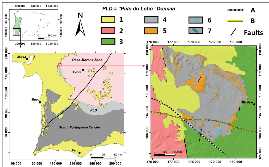
Figure 1. Geographical and geological context of the Pedreira da Engenbaria quarry. 1 - Mesozoic; 2 - “Pulo do Lobo” Domain; 3 - Carvalhal Formation; 4 and 5 - Cabrela Formation, respectively, Flysch and volcanic material; 6 - “Pedreira da Engenbaria” Formation; 7 - Other limestone outcrops within Cabrela Formation; A - Railroad; B - Highway.
