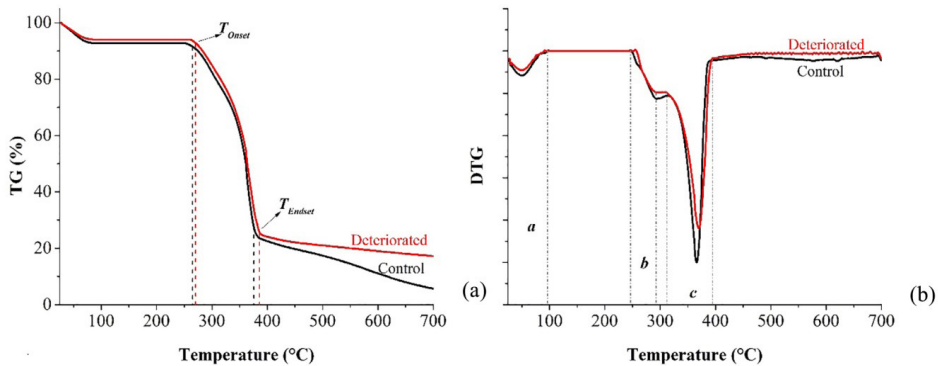
Figure 2: (a) TGA and (b) DTG curves of the woods of the control group and deteriorated by termites of Nasutitermes genus.
