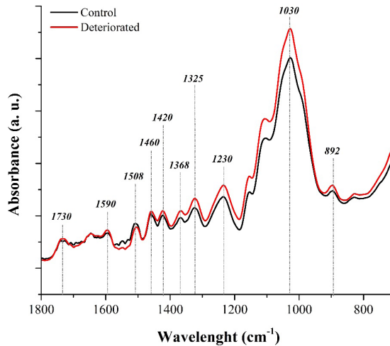
Figure 1: FTIR spectra of the woods of the control group and deteriorated by termites of Nasutitermes genus.
