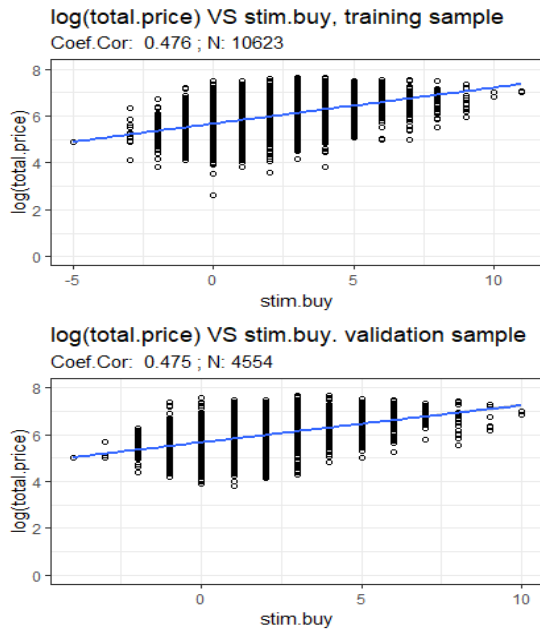
Figure 4. Scatter plots (with adjust lines) for log(total.price) vs stim.buy. Source: The Authors.
