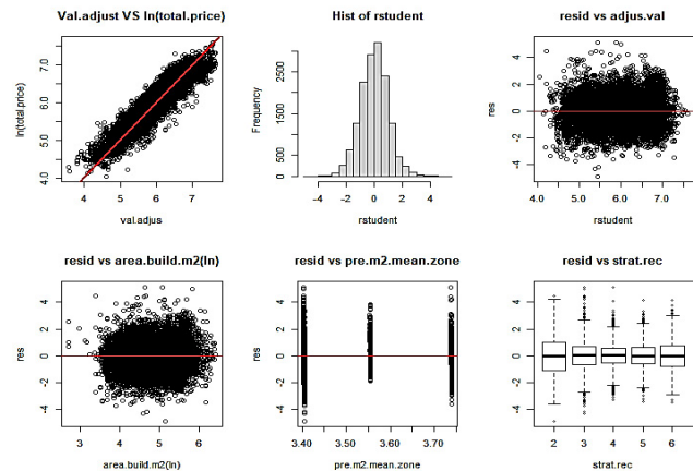
Figure 7. Analysis of residuals for regression in the complete sample, after exclusion of one property. N: 15,176 observations. Source: The Authors.
