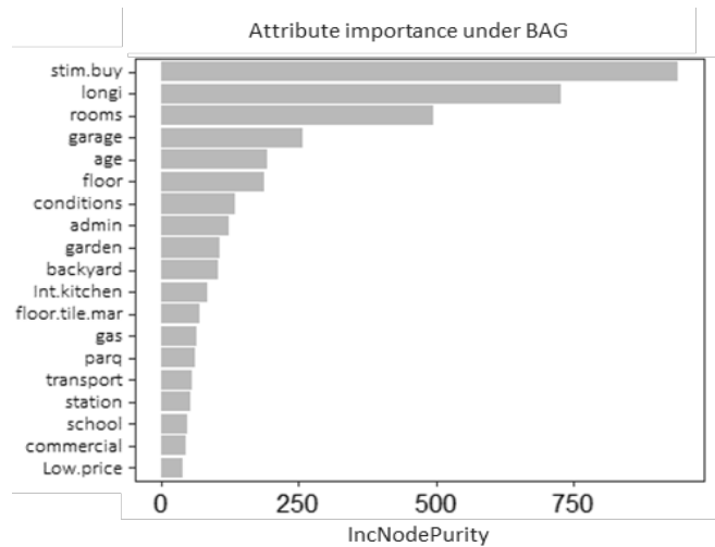
Figure 5. Importance of attributes in a trained bagging model, excluding the most important four attributes (top 4)
