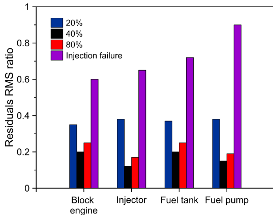
Figure 6. RMS residual signal acoustic
