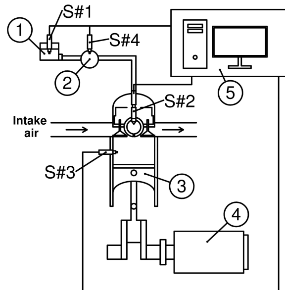
1. Diesel tank, 2. Gravimetric fuel meter, 3. Engine, 4. Dynamometer, 5. Data acquisition system.
