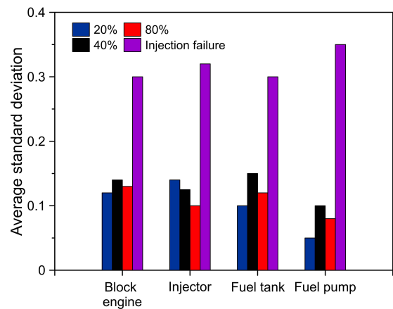
Figure 7. Standard deviation of the acoustic signal
