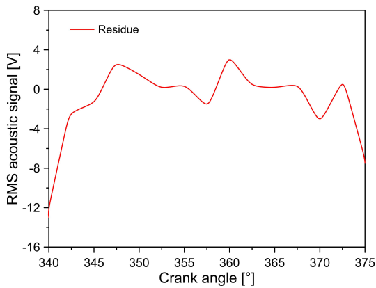
Figure 5. Residual acoustic signal with injector failure
