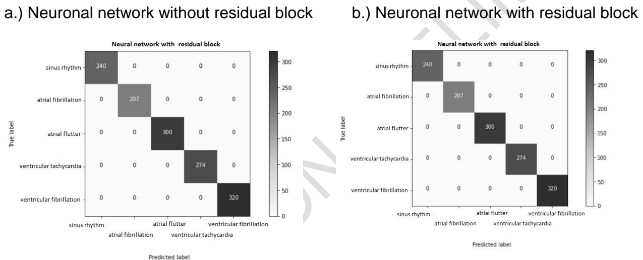
Figure 4. Confusion Matrices.
