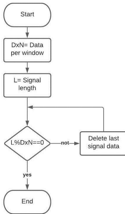
Figure 2. Algorithm to reduce the length of the windows.
