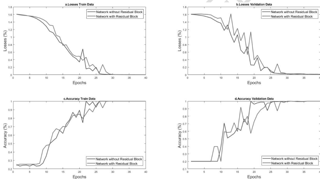
Figure 3. Training results.
