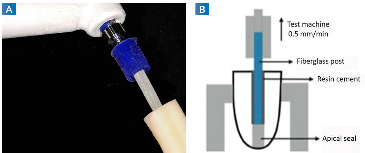
A: Sonic vibration (for 10 s) was applied with a specific tip placed on top of the post. B: Schematic configuration of the pull-out tests, performed using a universal testing machine at a crosshead speed of 0.5 mm/min.
