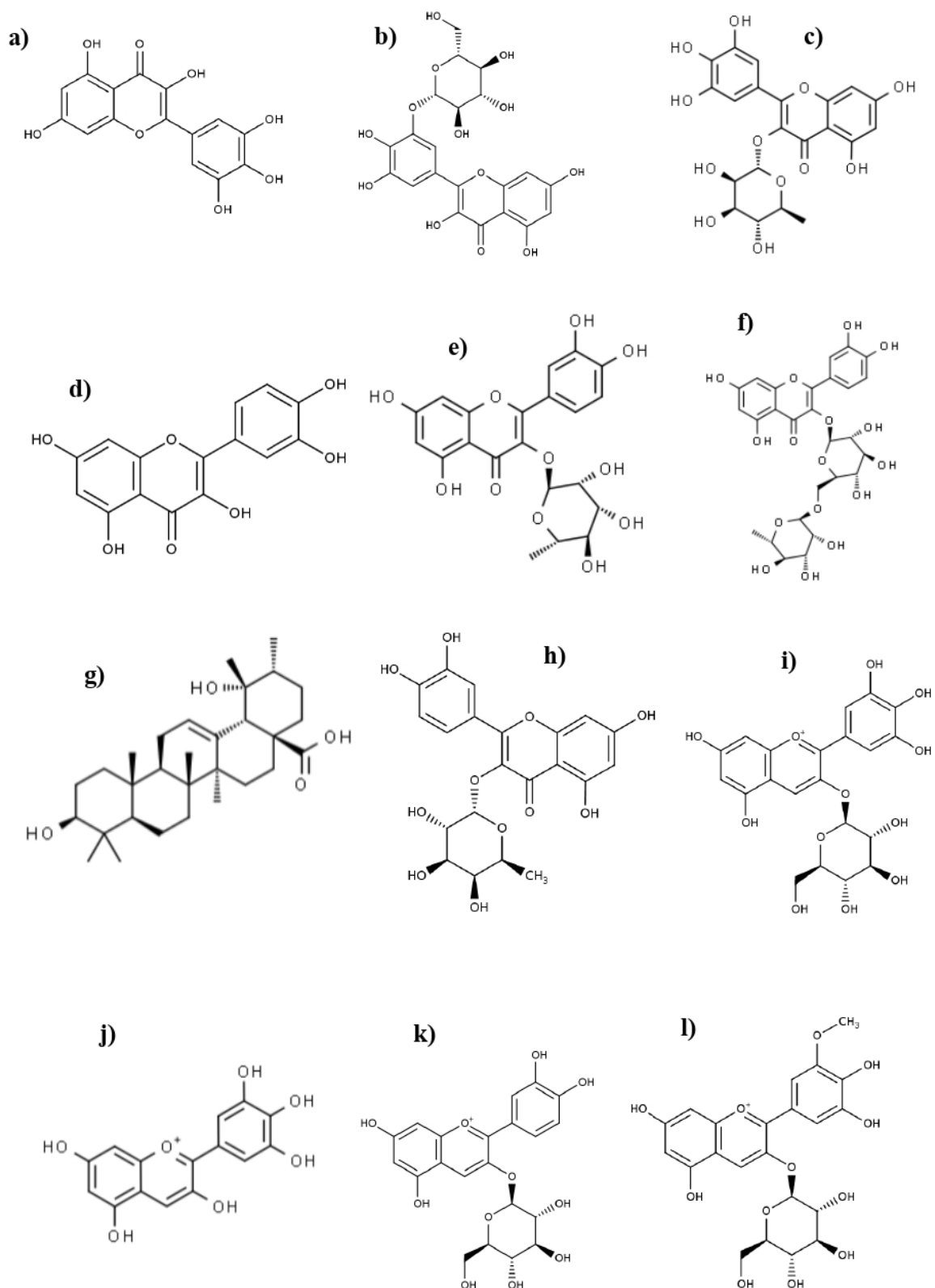
Figure 1. Main compounds isolated from C. icaco : a) Myricetin; b) Myricetin 3-O-glucuronide; c) Myricitrin; d) Quercetin; e) Quercitrin; f) Rutin; g) Pomolic acid; h) Quercetin 3-O-rhamnoside; i) Delphinidin-3-O-glucoside; j) Delphinidin; k) Cyanidin 3-glucoside; l) Petunidin-3-glucoside (Kim et al. , 2021; Neveu et al. , 2010).
