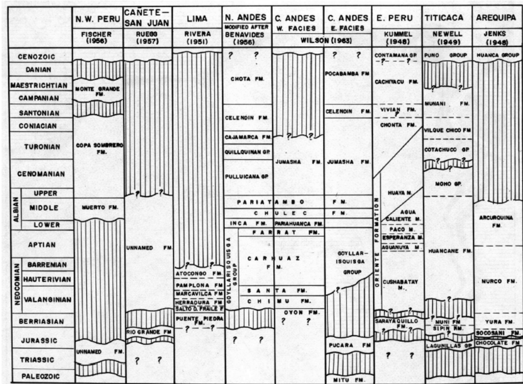
Figure 2. Correlation table for the Peruvian stratigraphic column (after Wilson, 1963).
