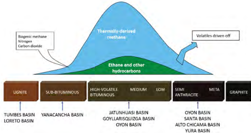
Figure 9. Gas Content in Basins according to the Coals.
