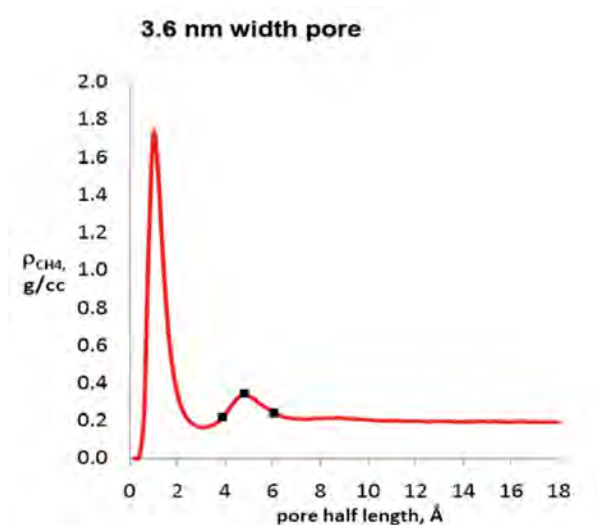
Figure 8. The density of the adsorbed methane phase. Source: LANGMUIR, I.; The Constitution and Fundamental Properties of Solids and Liquids, Journal of the American Chemical Society. Vol 38. 1996.
