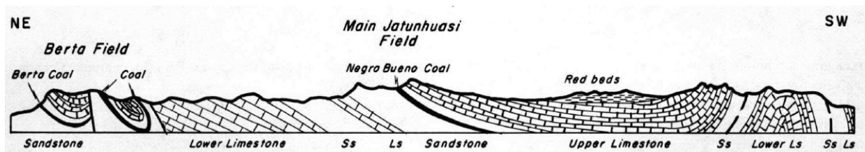
Figure 3. Diagrammatic cross-section through Jatunhuasi district viewed toward the southeast. No Scale. Length of section 10 to 12 km (After McLaughlin, 1922). Ls=Limestone; Ss=sandstone.
