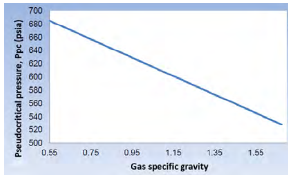
Figure 6. Pseudocritical Properties of Natural Gases, Pseudo critical Pressure. Source: The properties of petroleum fluids-McCain Williams second edition page 119.
