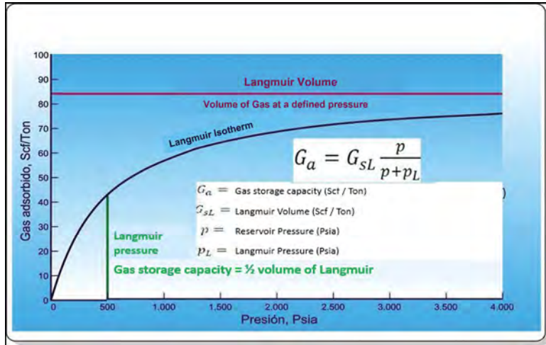
Figure 4. Langmuir adsorption isotherm
