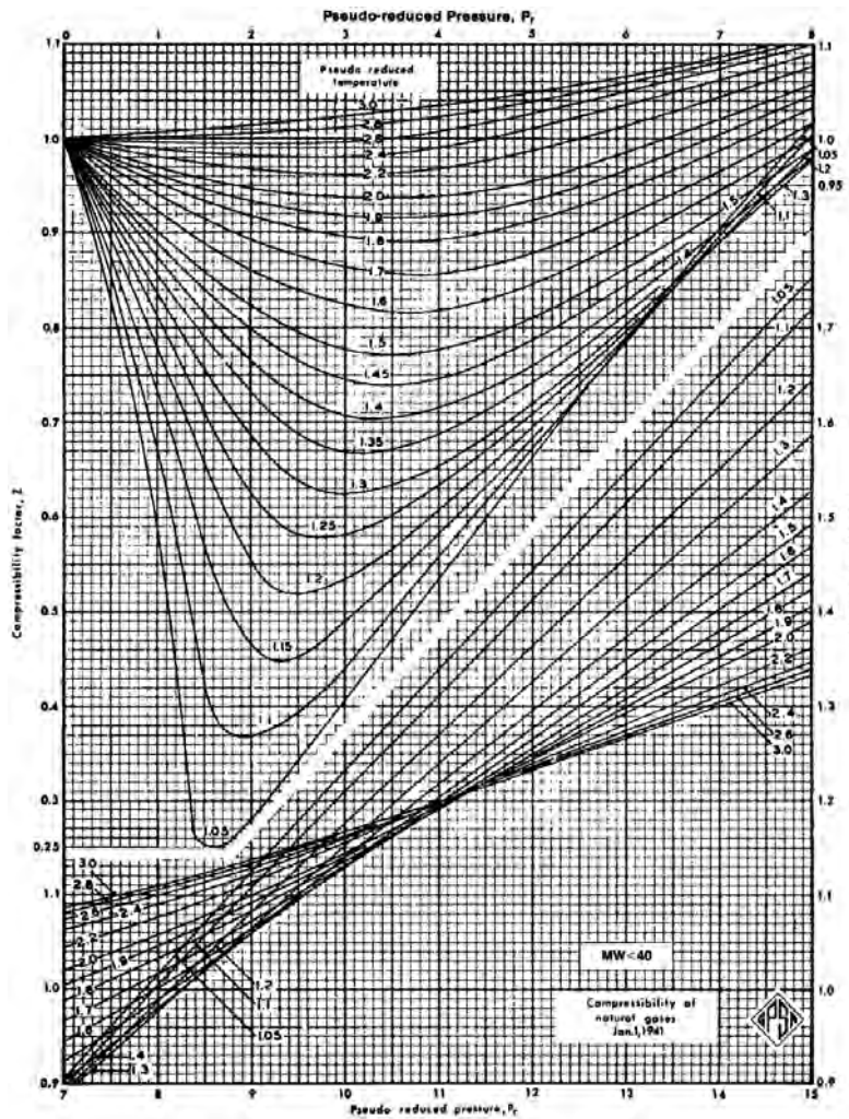
Figure 5. Compressibility factor for natural gases.
