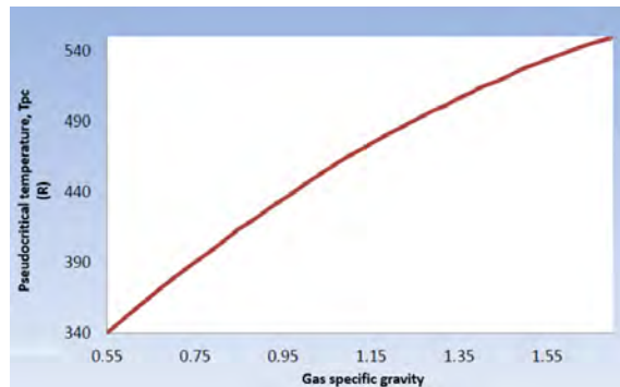
Figure 7. Pseudocritical Properties of Natural Gases, Pseudo critical Temperature Source: The properties of petroleum fluids-McCain Williams second edition page 119.
