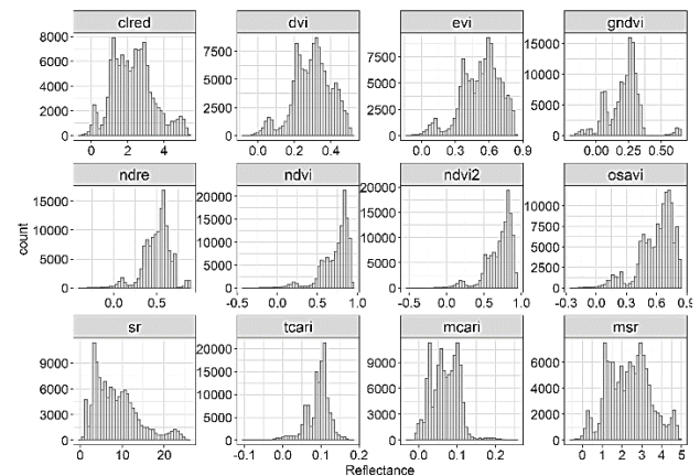
Figure 4. Histograms for VIs values of P. crassipes cover from monthly Sentinel images (September 2018 to March 2020) in the IHP. 'Clred' corresponds to Cl red edge index. Source: Authors.
