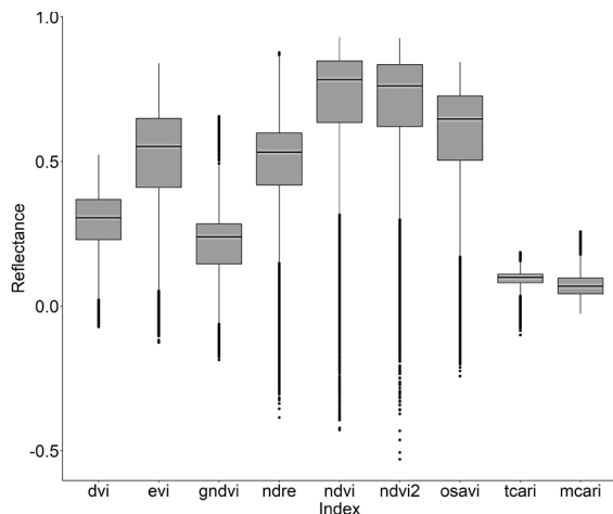
Figure 2. Boxplots for reflectance of small-scale VIs containing P. crassipes cover from monthly Sentinel images (September 2018 to March 2020) in the IHP. Source: Authors.
