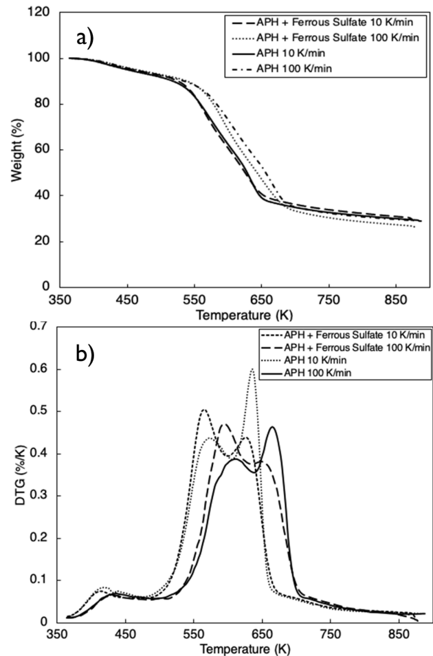
Figure 1. a) TG and b) DTG thermograms of APH and APH + 1% FeSO 4 at heating rates of 10 and 100 K/min, respectively Source: Authors
