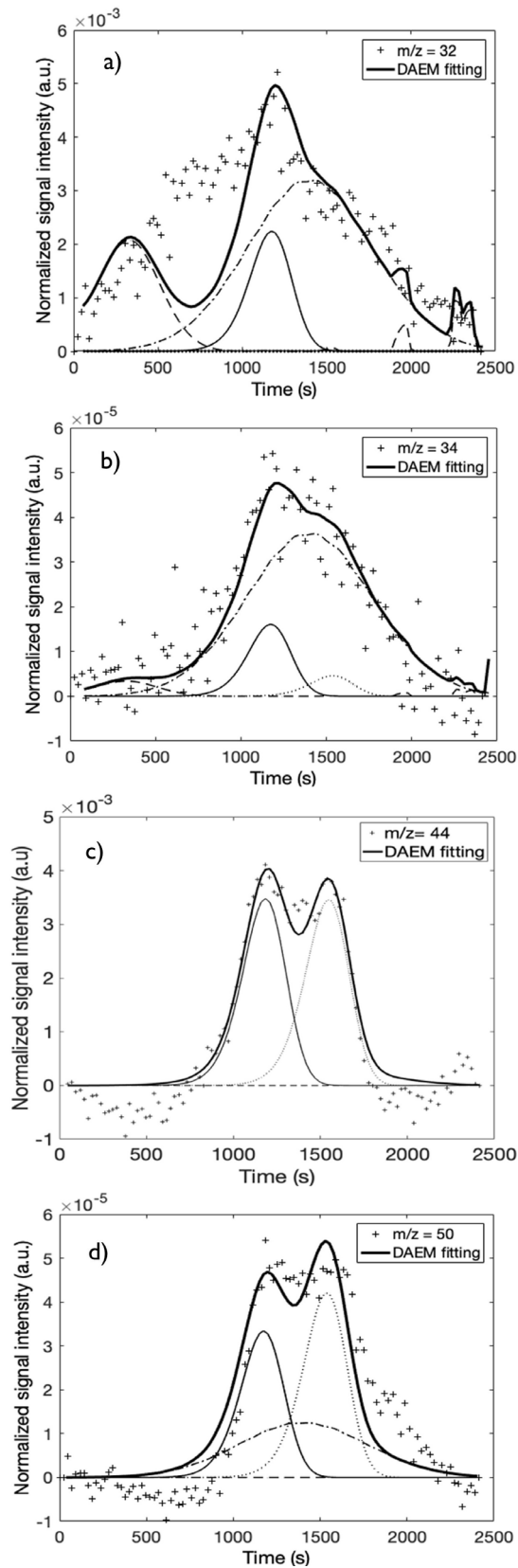
Figure 3. Fitting of the DAEM with four pseudo-components of selected m/z signal intensities: a) m/z = 32 , b) m/z = 34 , c) m/z = 44 , d) m/z = 50 of APH + 1% \text{FeSO}_3 at a 10 K/min heating rate
