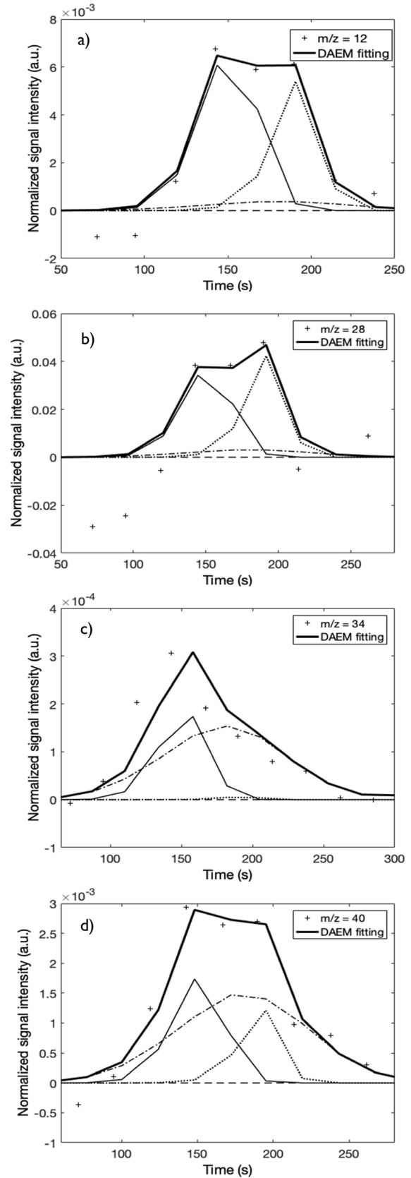
Figure 4. Fitting of the DAEM with four pseudo-components of selected m/z signal intensities: a) m/z = 12 , b) m/z = 28 , c) m/z = 34 , d) m/z = 40 of APH + 1% \text{FeSO}_3 at a 100 K/min heating rate
