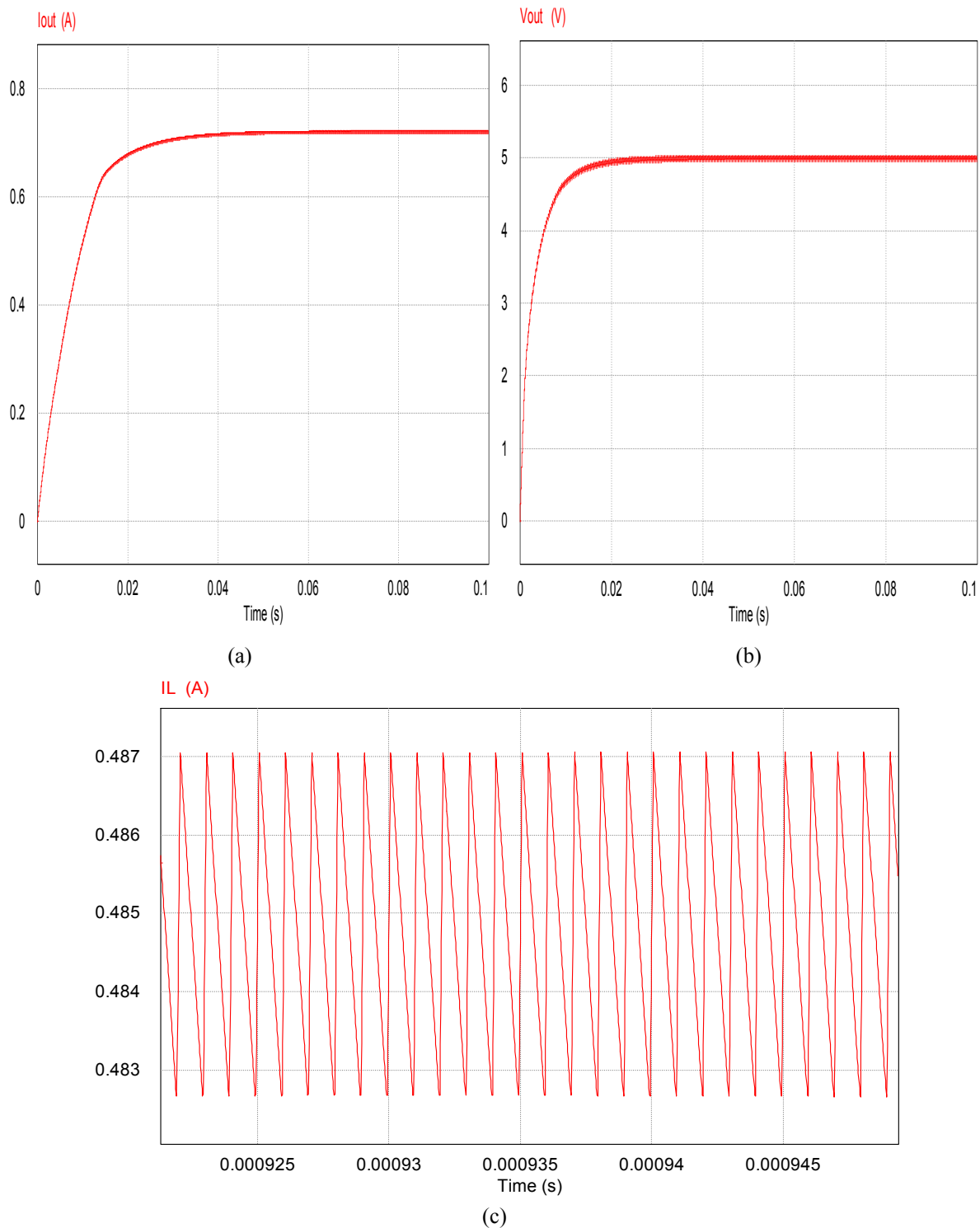
Fig. 10. Waveforms in boost converter, (a) Output current, (b) Output voltage, (c) Current flowing in the spiral inductor
