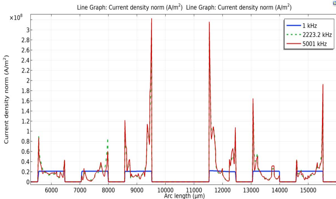
Fig. 7. Simulations of the current density norm according to the arc length mentioned in spiral inductor
