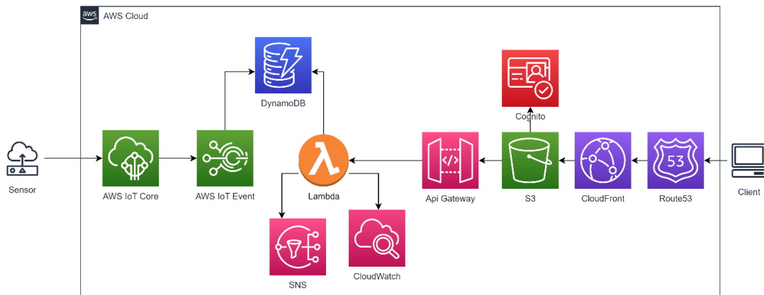
Figure 3 Solution reference design in AWS
