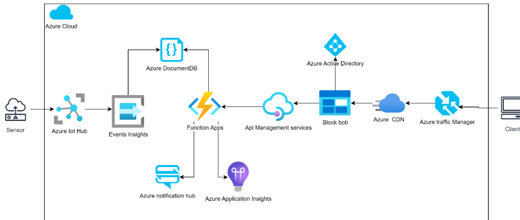
Figure 4. Azure solution reference design.
