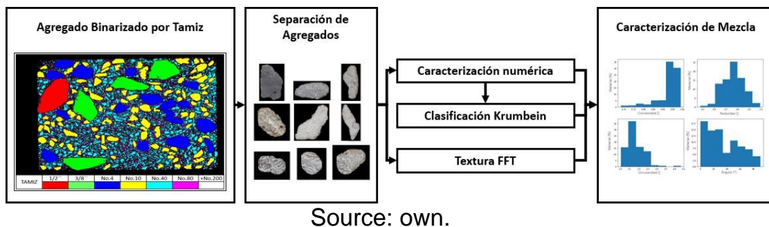
Figure 18. Flow of description of the aggregate.
