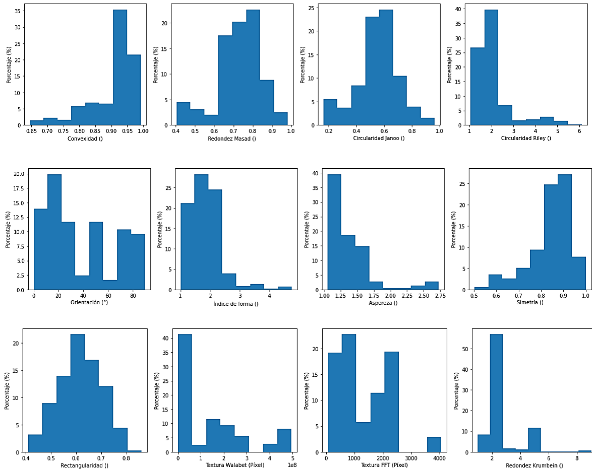
Figure 13. Characterization of the aggregate inside of the mix.
