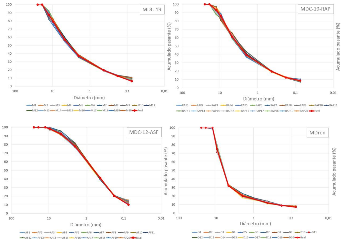
Figure 11. Reconstruction granulometric.
