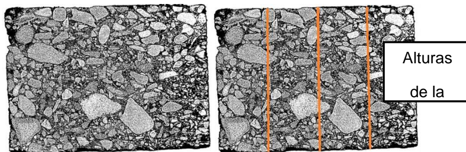
Figure 3. Binarization and taking heights mix MDC-19-RAP.
