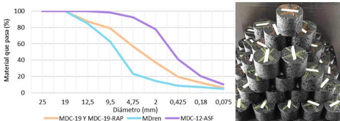
Figure 2. Granulometric curves and manufacturing of asphalt mixtures.
